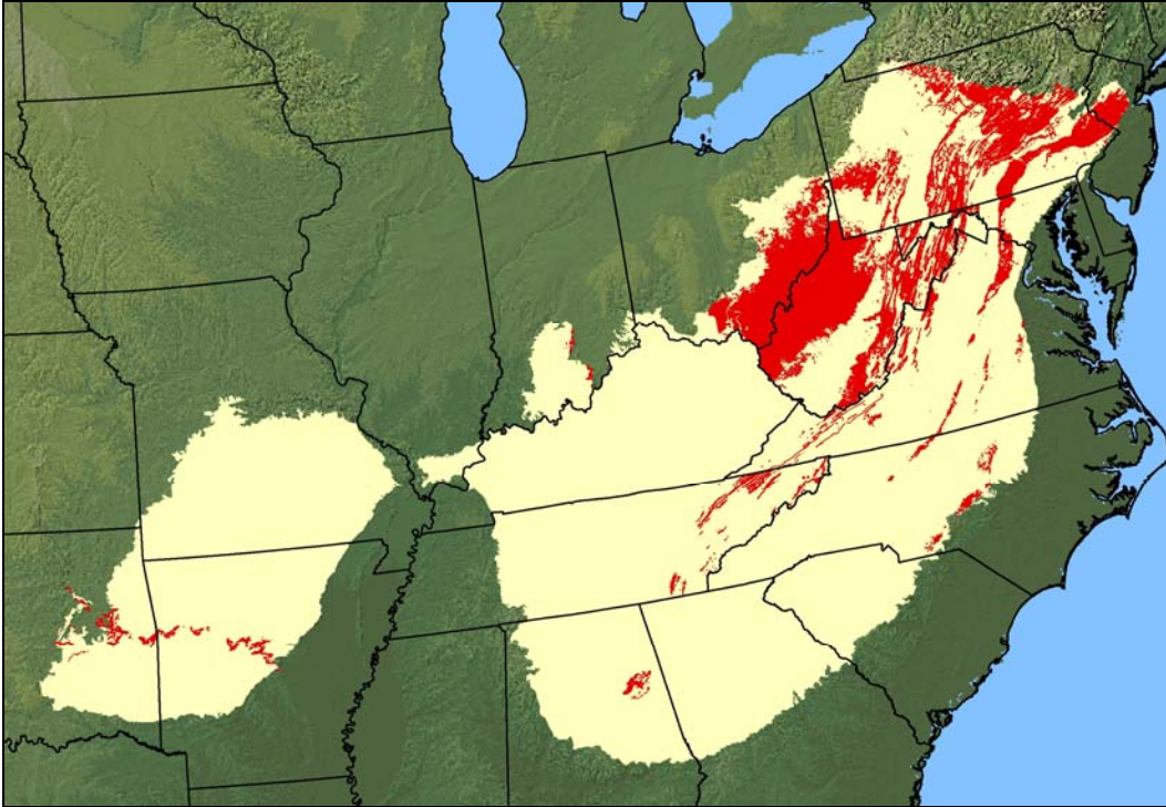
Figure 34. Locations of soils derived from red parent materials (red areas) in the Eastern Mountains and Piedmont Region. The map was developed using NRCS soil survey (SSURGO) data and depicts map units that contain at least one soil component derived from red parent materials.
