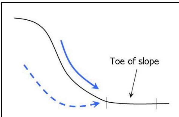
Figure 6. At the toe of a hill slope, the gradient is only slightly inclined or nearly level. Blue arrows represent flow paths of surface water (solid arrow) and groundwater (dashed arrow).
