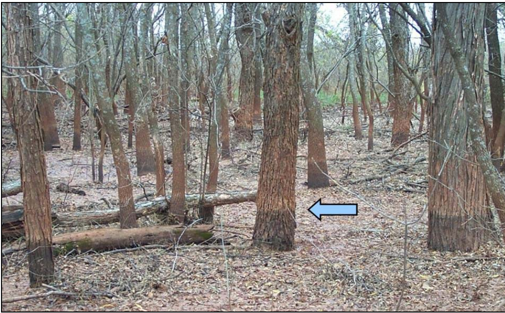
Figure 38. Water marks (dark stains) on trees in a seasonally flooded wetland. The top of one water mark is indicated by the arrow.
